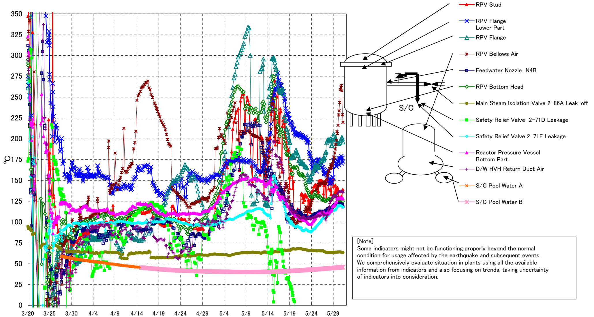
Fukushima Daiichi Nuclear Power Station Unit3 Parameters of Temperature (Typical Points)
